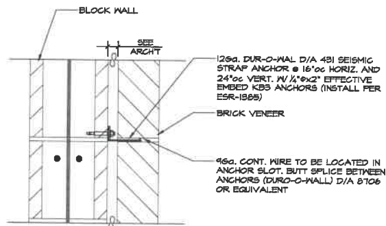
ALTERNATE VENEER TIE
