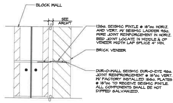
TYPICAL VENEER TIE
